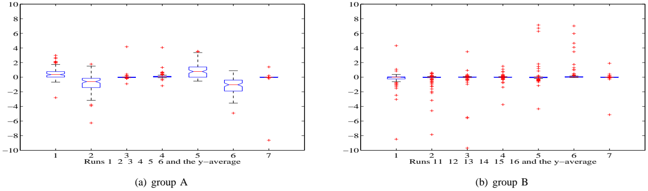
Fig. 4. Bar plots of the relative residuals of the original (gridded) data against the spline fit for \ell = 5 (outliers outside [-10\%, 10\%] are not shown)
