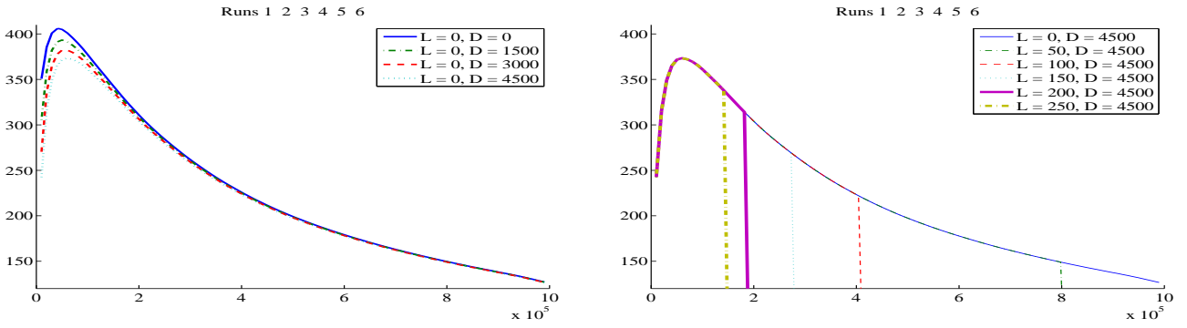
Fig. 5. Average performance P_{ave} plots for group A depending on the rejuv. point: varied numbers of dropped requests during rejuv. D (left, for L = 0 ) and varied SLA levels L (right, for D = 4500 )
