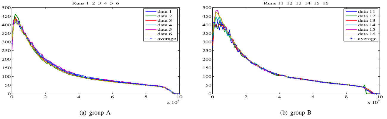
Fig. 2. Server performance versus number of served requests: original (gridded) data and the y -averages
