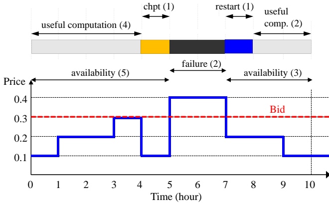
Fig. 2. Illustration of the execution model and computation of the random variables (RVs)
