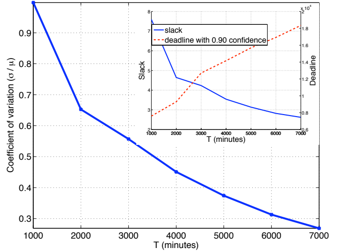
Fig. 6. Outer: Coefficient of variation of execution as task length T increases with bid price u_b=0.80 . Inner: Slack and deadline as T increases
