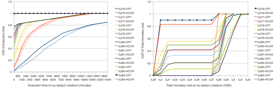
Fig. 9. CDF of execution time ( ET , left) and monetary cost ( M , right) for task length of T = 246 minutes on instance type A (workload W1)
