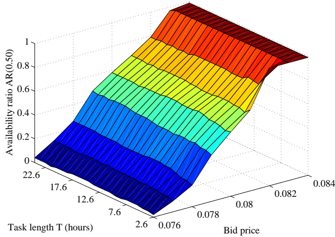
Fig. 5. Availability ratio AR(p) for p = 0.5 (median) (left) and for p = 0.9 (right) depending on the bid price and the task length T
