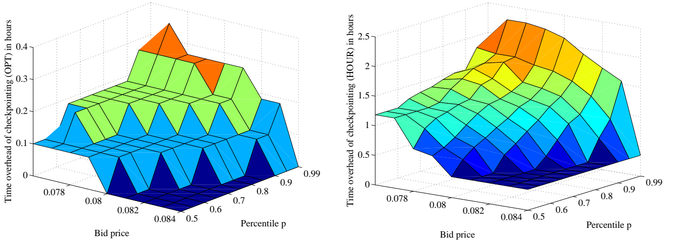
Fig. 4. Overhead ( AT(p) - T ) of the checkpointing for the strategy OPT (left) and HOUR (right) for various bid prices and percentiles p
