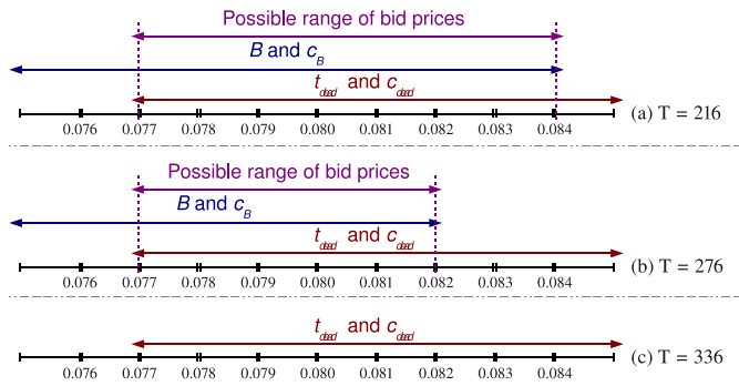
Fig. 8. The ranges of the bid prices according to the results in Figure 7
