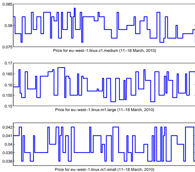
Fig. 1. Price history for some Spot Instance types (in USD per hour; geographic zone eu-west ; operating system Linux/UNIX)
