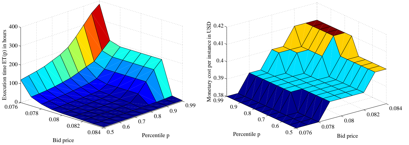
Fig. 3. Influence of bid price and percentile p on the execution time ET(p) (left) and monetary cost per instance M(p) (right) ( p corresponds to confidence c_{dead} for ET and to confidence c_B for M )
