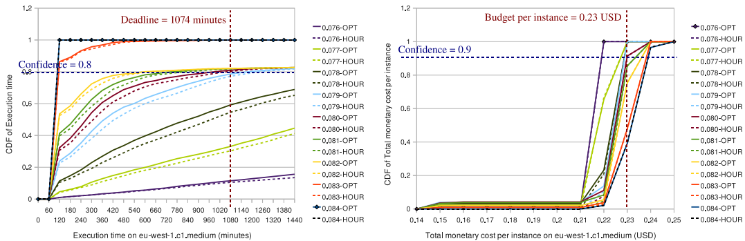
Fig. 10. CDF of execution time ( ET , left) and monetary cost ( M , right) for task length of T = 164 minutes on instance type A (workload W2)
