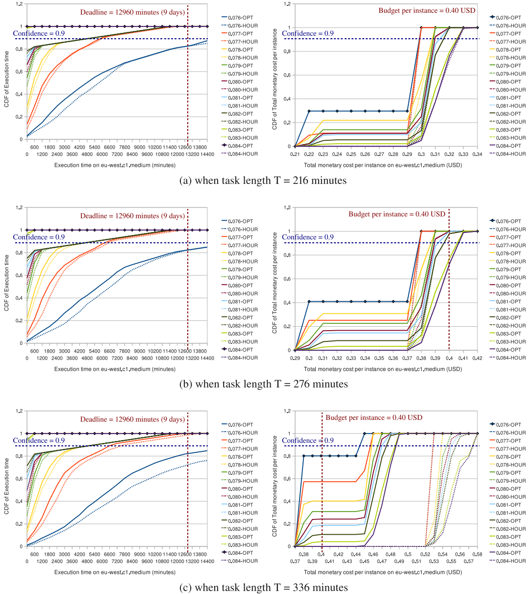
Fig. 7. CDF of execution time ( ET , left) and monetary cost ( M , right) for various task lengths on instance type A (workload W1)
